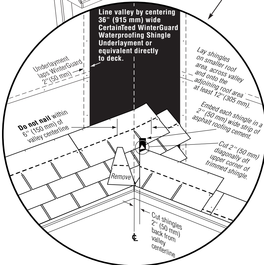
Figure 10-11: Highlight of closed-cut valley details.
