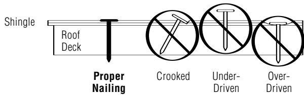
Figure 10-2: Proper and improper nailing.
