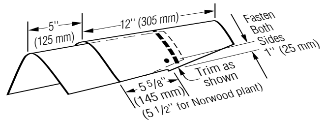
Figure 10-25: Installation of caps along the hips and ridges.
