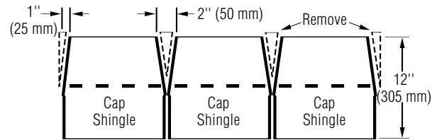
Figure 10-24: Cut tabs, then trim back to make cap shingles (English dimensions shown).
