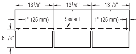
Figure 10-3: Use four nails for every full shingle.
