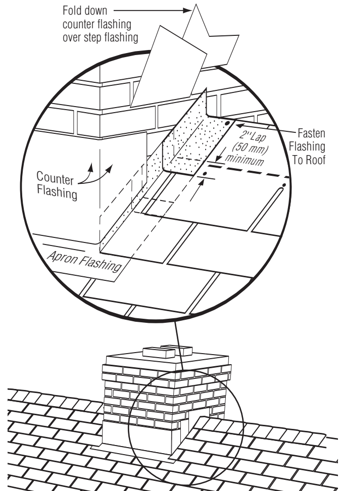
Figure 10-18: Flashing around a chimney.
