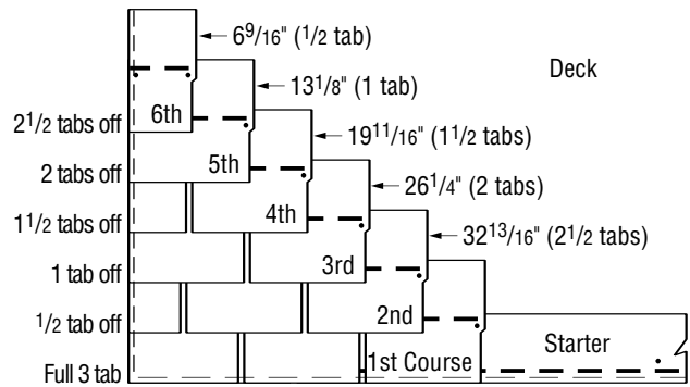
Figure 10-17: Half-Tab Method.
