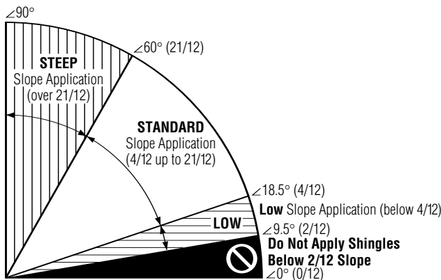
Figure 10-1: Slope definitions.
