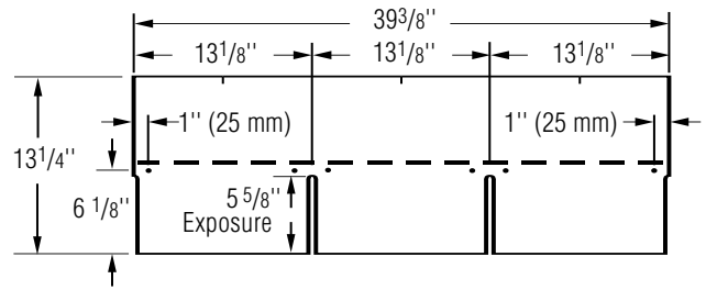
Figure 10-5: Six nails can be used for high wind applications.
