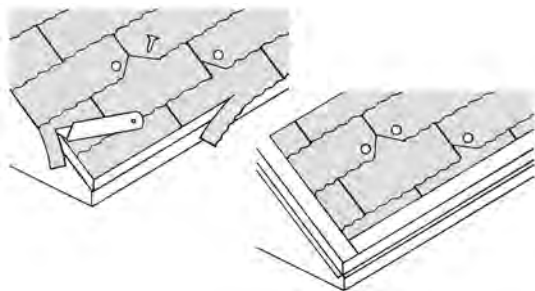
Figure 10-19: Preparing an old roof for reroofing.
