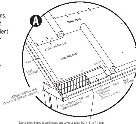
Extend the shingles above the rake and save at about 1/2" (13 mm) if drip edge is used or about 3/4" (19 mm) if no drip edge is used.
